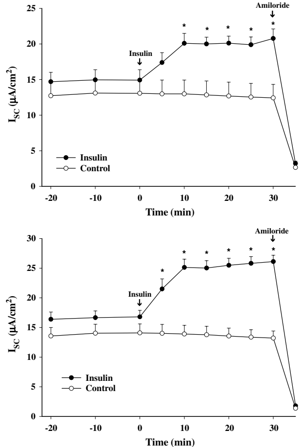
Fig. 2. Insulin-induced Na^+ I_{SC} in renal principal epithelial cells. Insulin ( 100 \text{ nM} ) was added to the serosal bathing media of monolayers formed by either the mpkCCD cl4 (upper panel) or A6 cell line (lower panel) at time = 0 \text{ min} . Amiloride ( 10 \mu M ) was added to the apical bathing media 30 min following insulin stimulation. Symbols represent the mean of n experiments \pm SEM. As determined by Student's t test, insulin induced a significant increase in reabsorptive Na^+ flux beginning at 10 and 5 min post-hormone addition in mpkCCD cl4 ( n = 6 ) and A6 ( n = 7 ) cells, respectively. *p \leq 0.05 .
